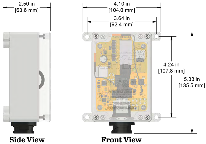
Figure 1. Dimensions
