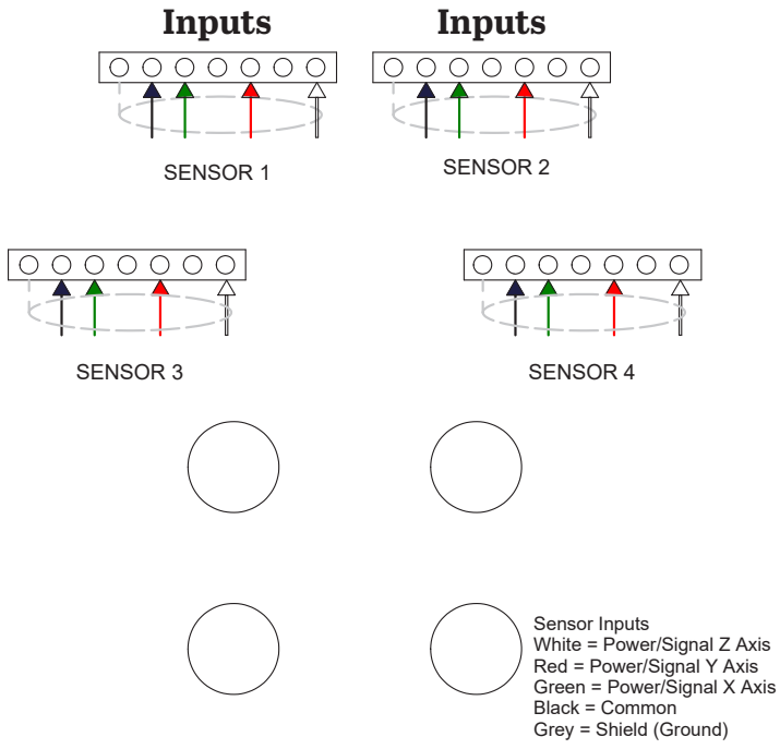
Figure 10. Field Wiring for Four-Conductor Triaxial Sensor Inputs
