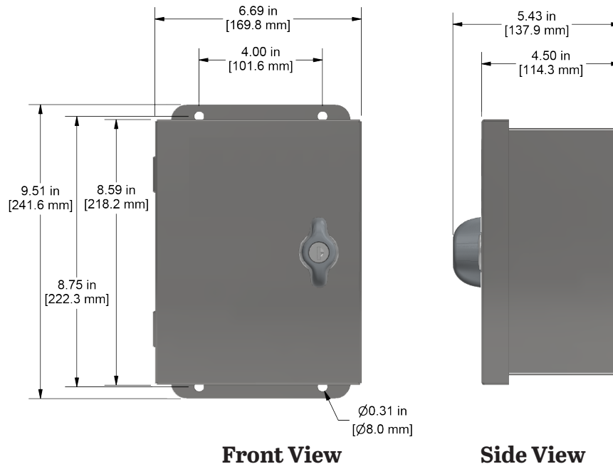
Figure 1. Dimensions
