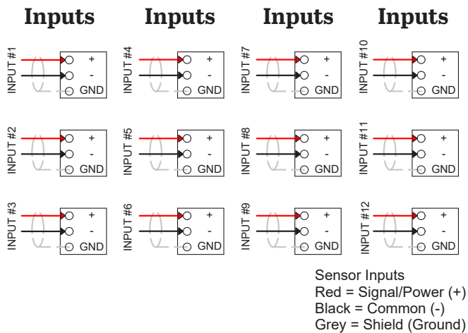
Figure 10. Connecting Cables to Modular Switch Box (SSB1002)
