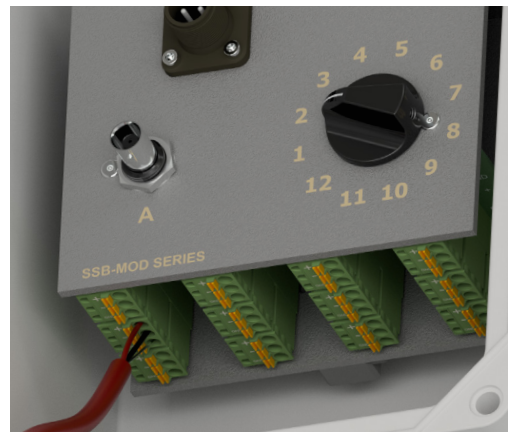
Figure 10. Connecting Cables to Modular Switch Box (SSB1002)
