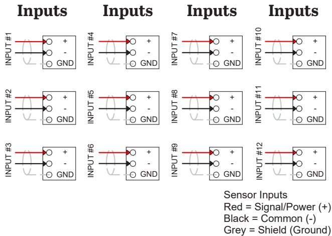
Figure 10. Connecting Cables to Modular Switch Box (SSB2002)
