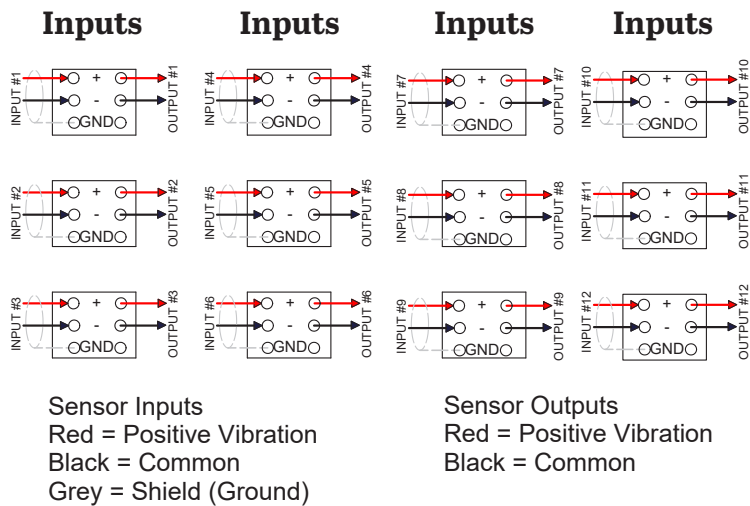
Figure 11. Connecting Cables to Modular Switch Box (SSB2003)
