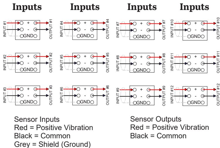
Figure 11. Connecting Cables to Modular Switch Box (SSB3001)
