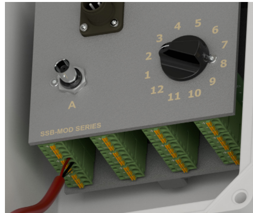
Figure 10. Connecting Cables to Modular Switch Box (SSB3000)
