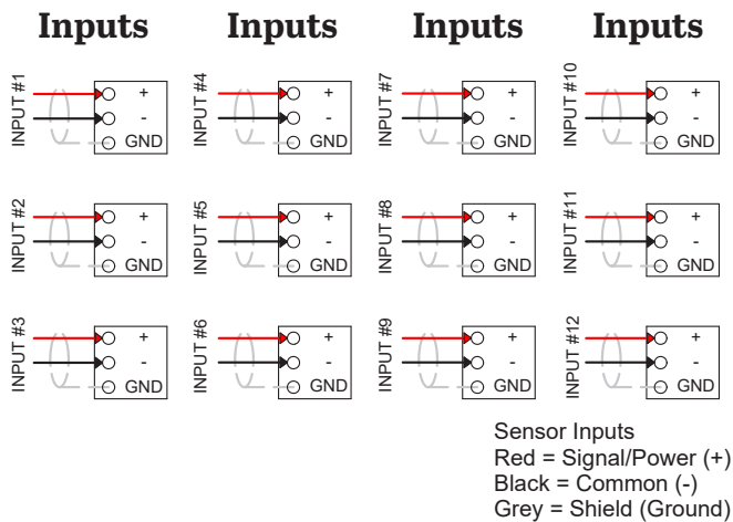
Figure 10. Connecting Cables to Modular Switch Box (SSB3000)
