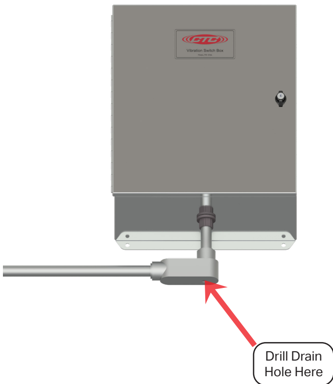
Figure 4. Conduit Entry for Switch Box
