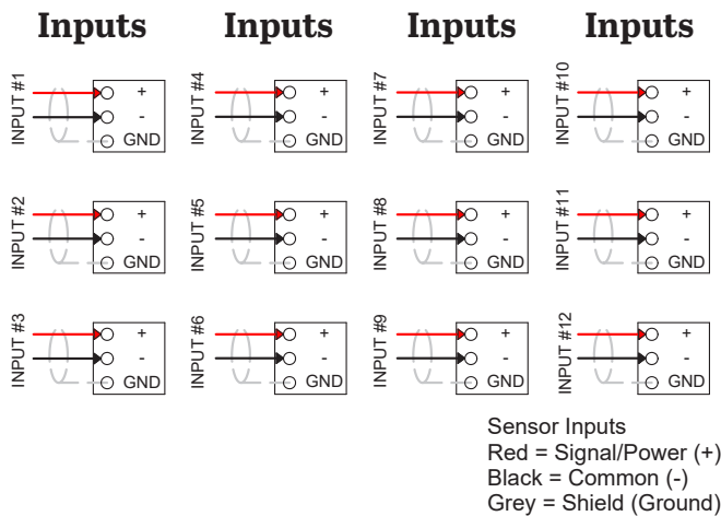
Figure 10. Connecting Cables to Modular Switch Box (SSB4000)
