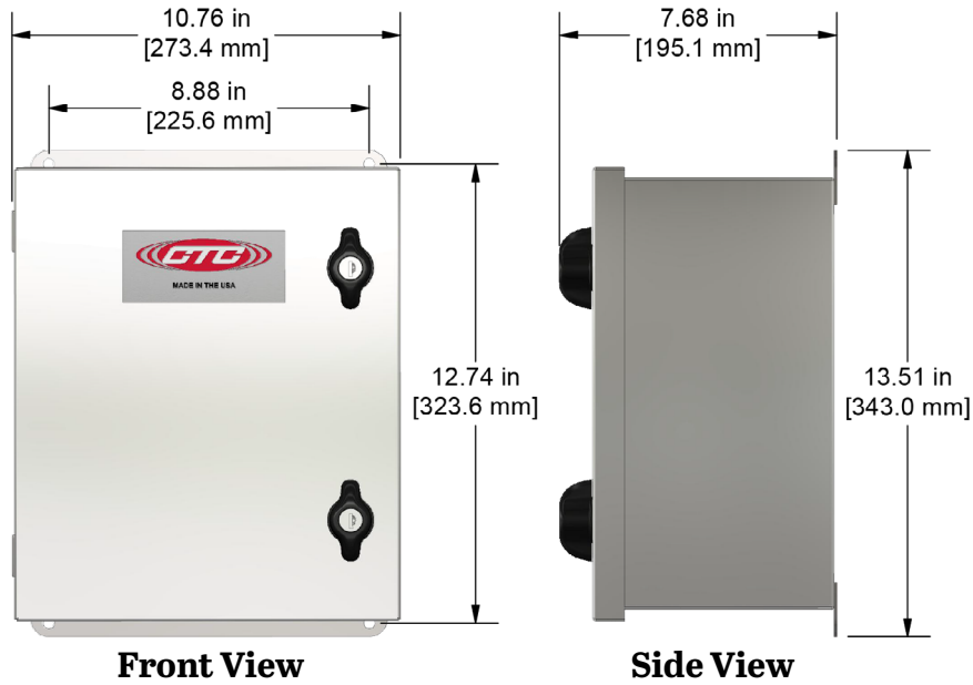
Figure 1. Dimensions
