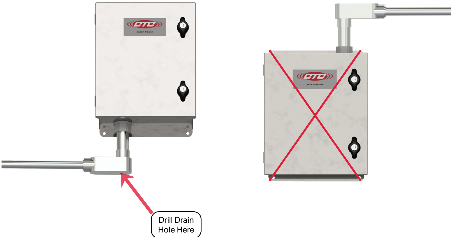
Figure 4. Conduit Entry for SCE200 Series
