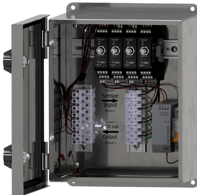
Figure 2. Diagram
