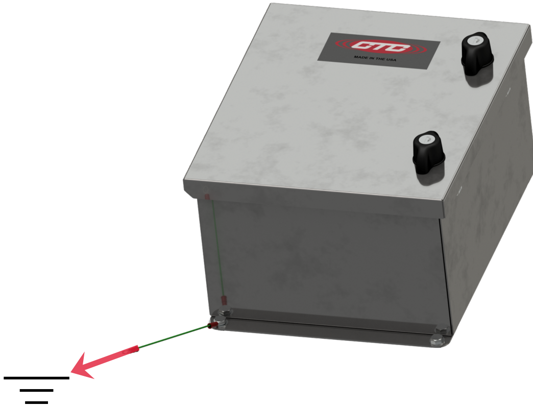
Figure 6. Ground Wire Placement
