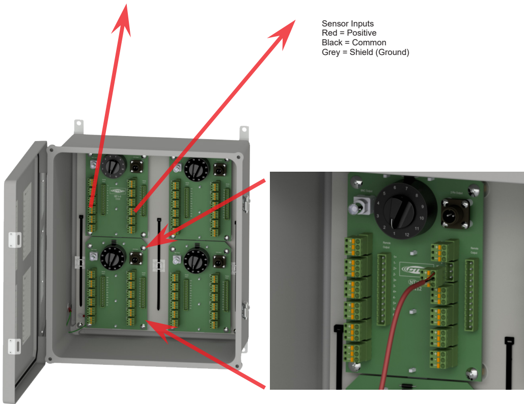
Figure 10. Field Wiring for 2-Conductor Sensor Inputs
