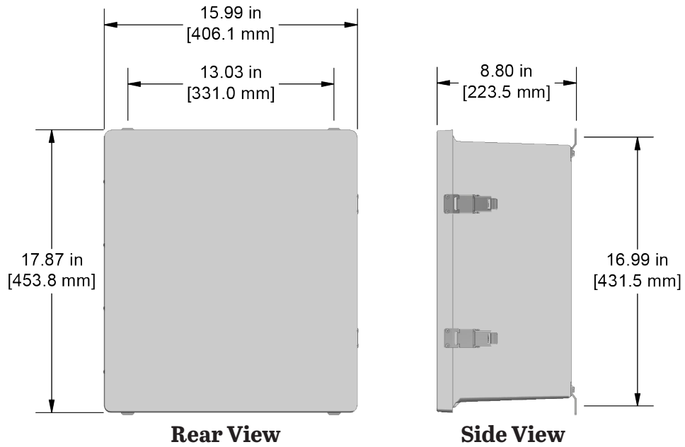
Figure 1. Dimensions
