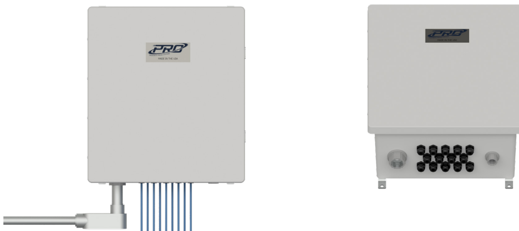
Figure 6. Cable Exit
