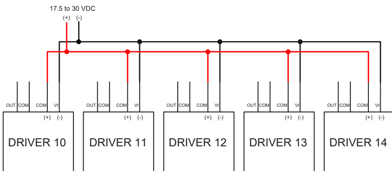
Figure 7. Wiring Diagram
