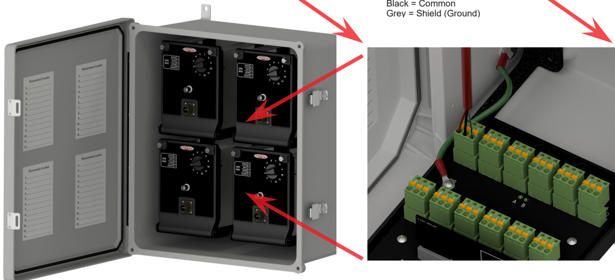
Figure 10. Connecting Cables to Switch Box
