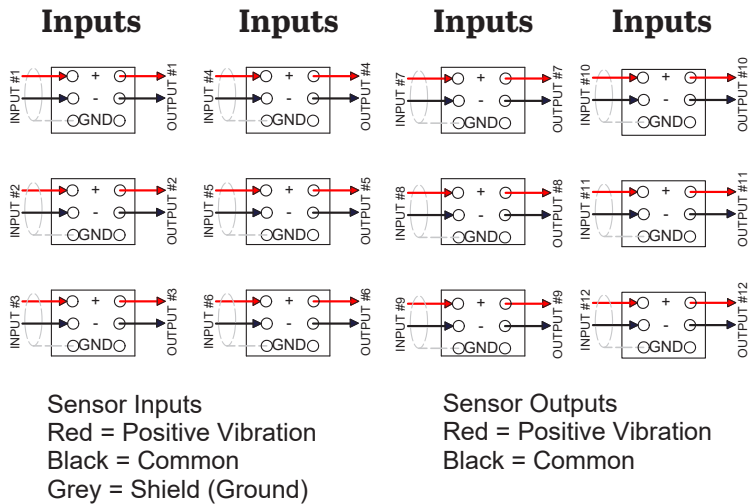
Figure 11. Connecting Cables to Modular Switch Box (SSB6001)
