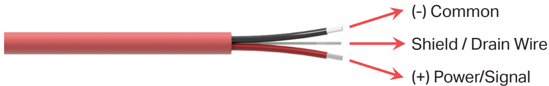
Figure 9. Stripped Wire
