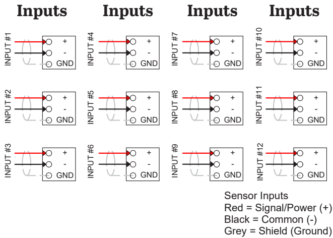
Figure 10. Connecting Cables to Modular Switch Box (SSB6000)
