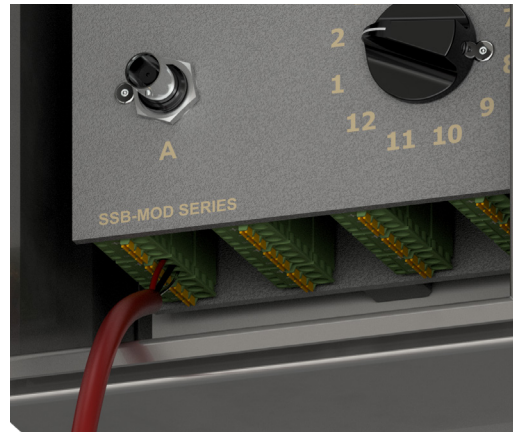
Figure 10. Connecting Cables to Modular Switch Box (SSB6000)
