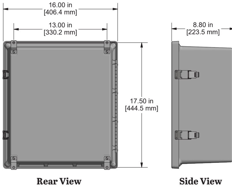
Figure 1. Dimensions
