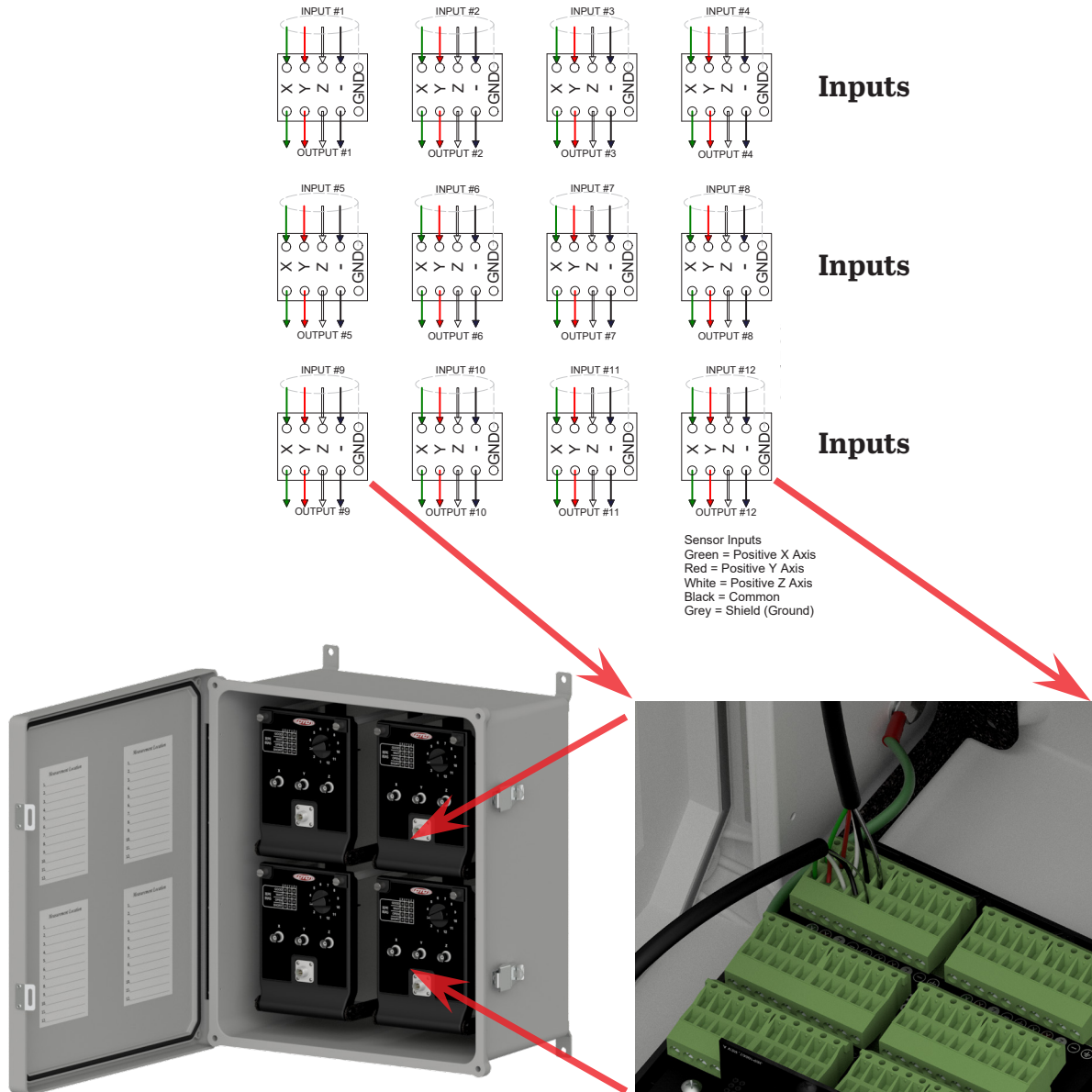
Figure 11. Field Wiring for Continuous Output
