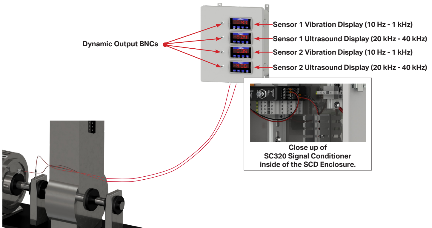
Diagram showing two Ultrasound sensors mounted on bearing housings, attached to connectors with cabling running into the bottom of the SCD Enclosure.
