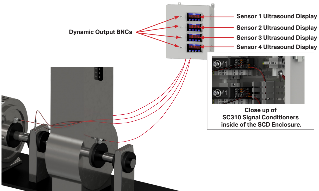
Diagram showing four Ultrasound sensors mounted on bearing housings, attached to connectors with cabling running into the bottom of the SCD Enclosure.
