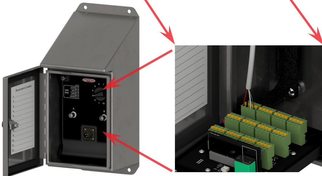
Figure 10. Field Wiring for 3-Conductor Sensor Inputs
