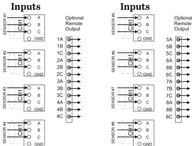
Figure 10. Field Wiring for 3-Conductor Sensor Inputs
