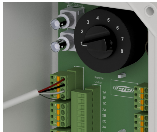
Figure 10. Field Wiring for 3-Conductor Sensor Inputs
