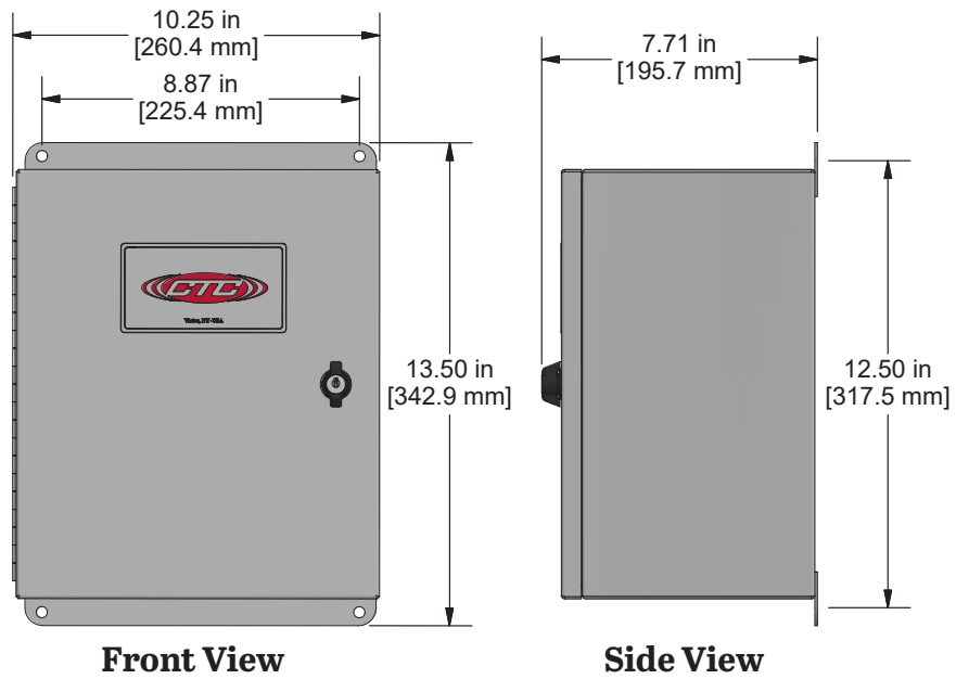
Figure 1. Dimensions
