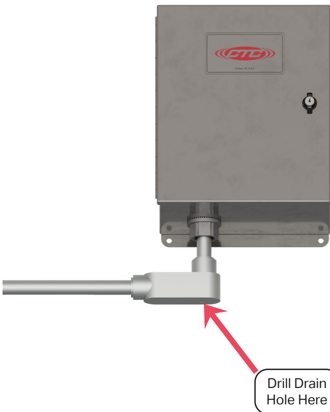
Figure 4. Conduit Entry for SCE200 Series
