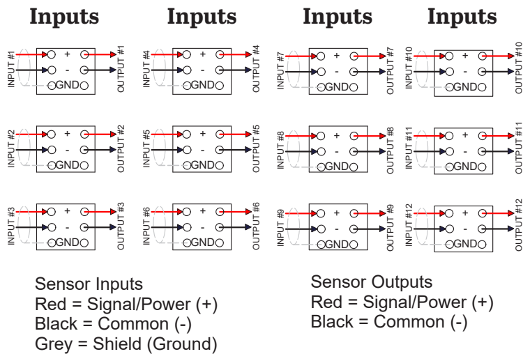
Figure 11. Connecting Cables to Modular Switch Box (SSB2001)
