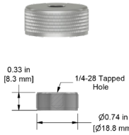
MH110-1A Ultra low profile, pull strength: 21 lbs (10 kg)
