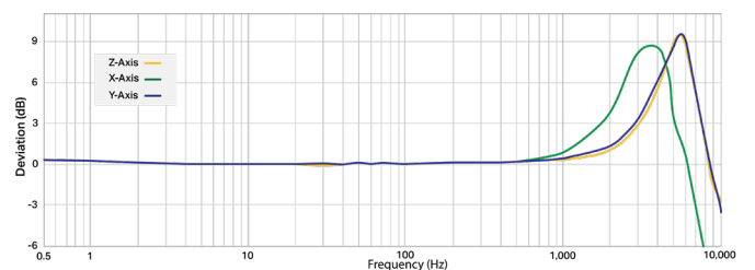
WS300 Series ConnectSens Wireless Sensor - Triaxial Dynamic Vibration Signal Capture with Temperature Output
