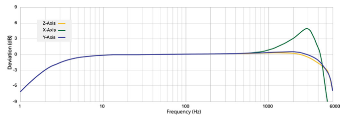
WS100 Series ConnectSens Wireless Sensor - Triaxial Overall Vibration Signal with Temperature Output
