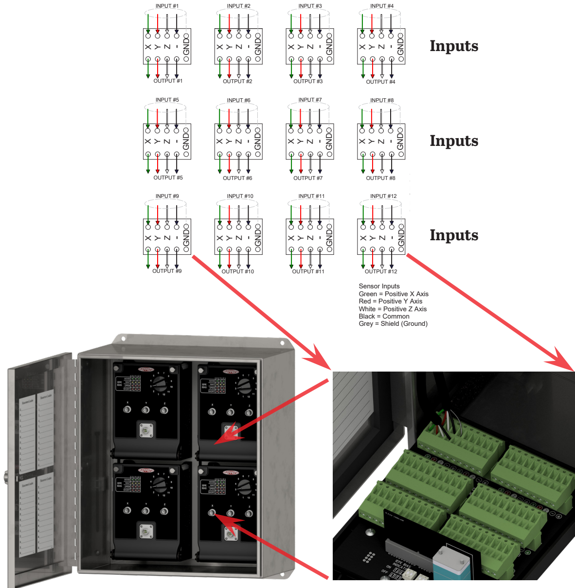
Figure 11. Field Wiring for Continuous Output
