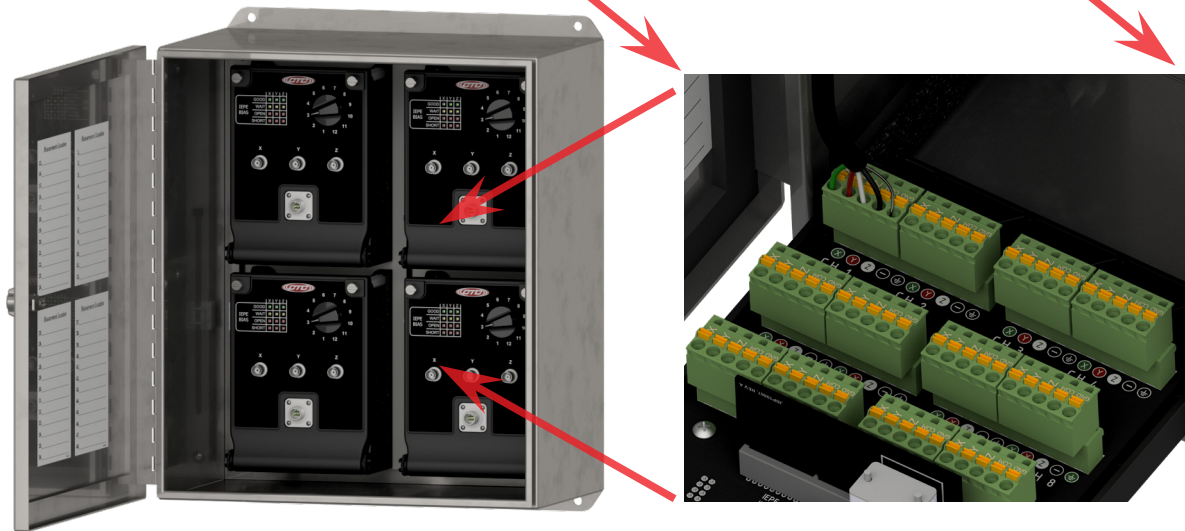
Figure 10. Field Wiring for 4-Conductor Triaxial Sensor Inputs
