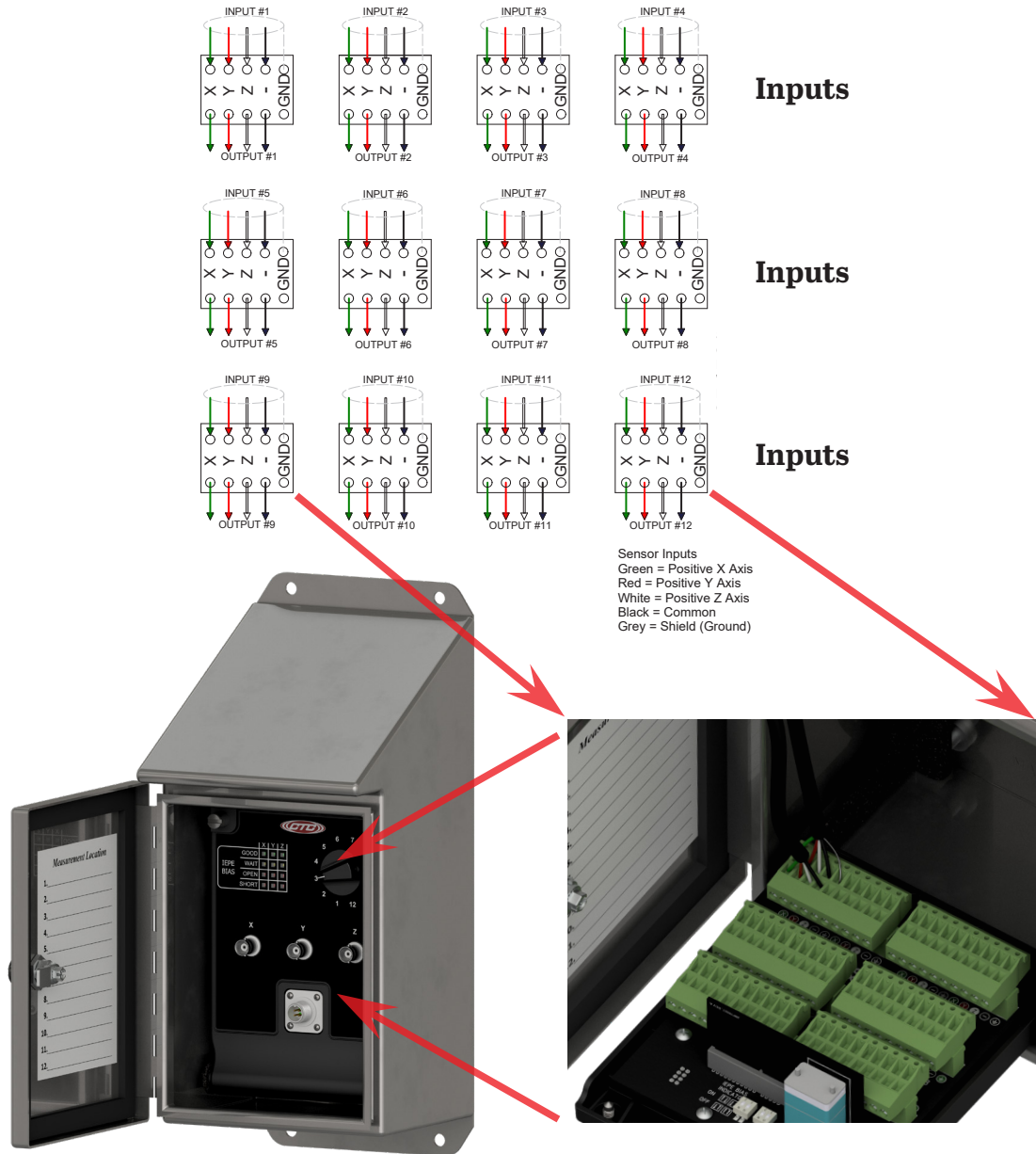
Figure 11. Field Wiring for Continuous Output
