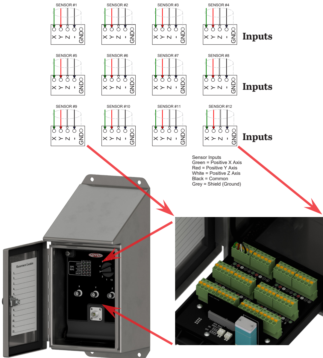
Figure 10. Field Wiring for 4-Conductor Triaxial Sensor Inputs
