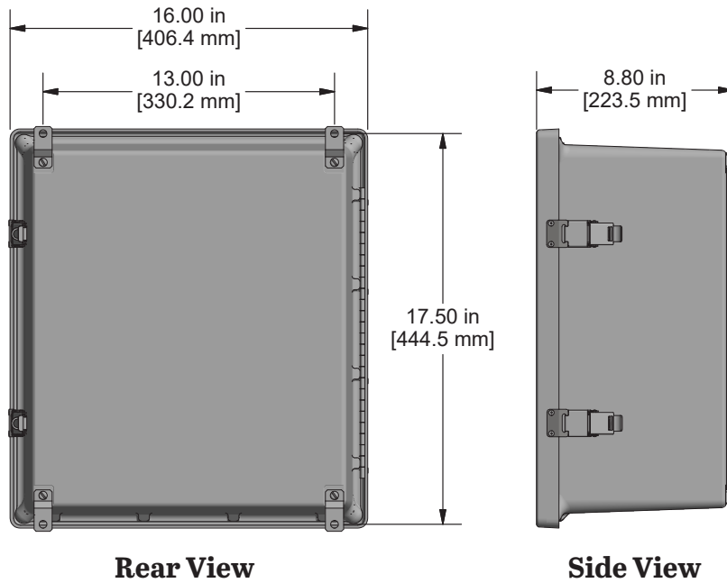
Figure 1. Dimensions
