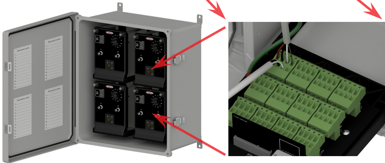
Figure 11. Field Wiring for Continuous Output
