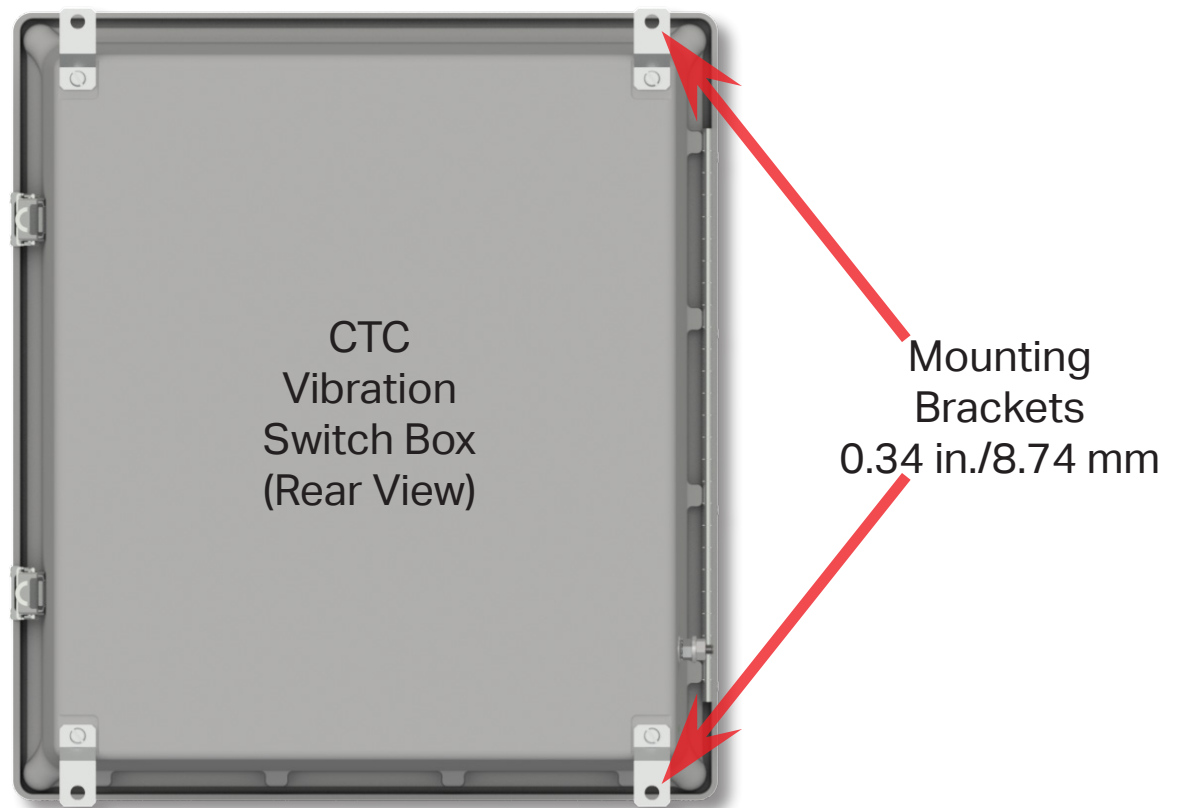
Figure 3. Mounting Bracket Placement
