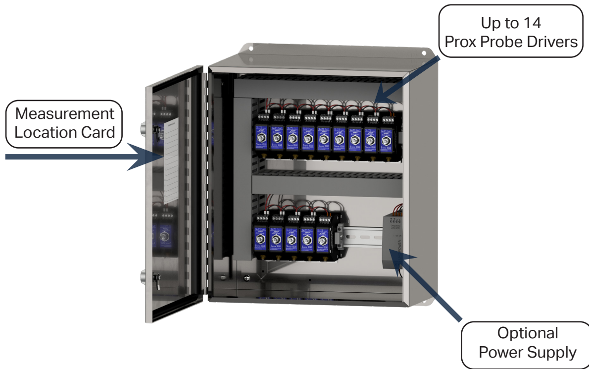
Figure 2. Diagram
