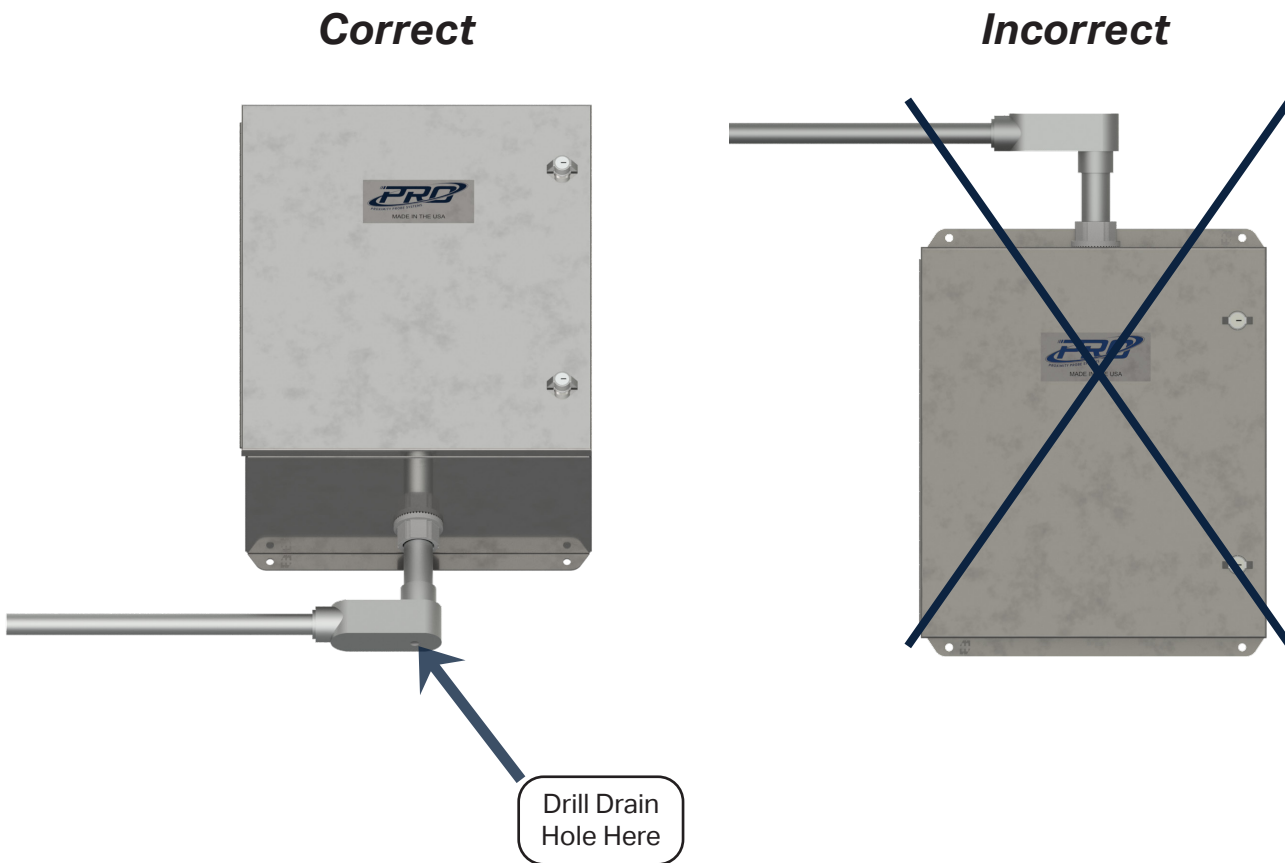
Figure 4. Conduit Entry for Proximity Probe Driver Enclosure
