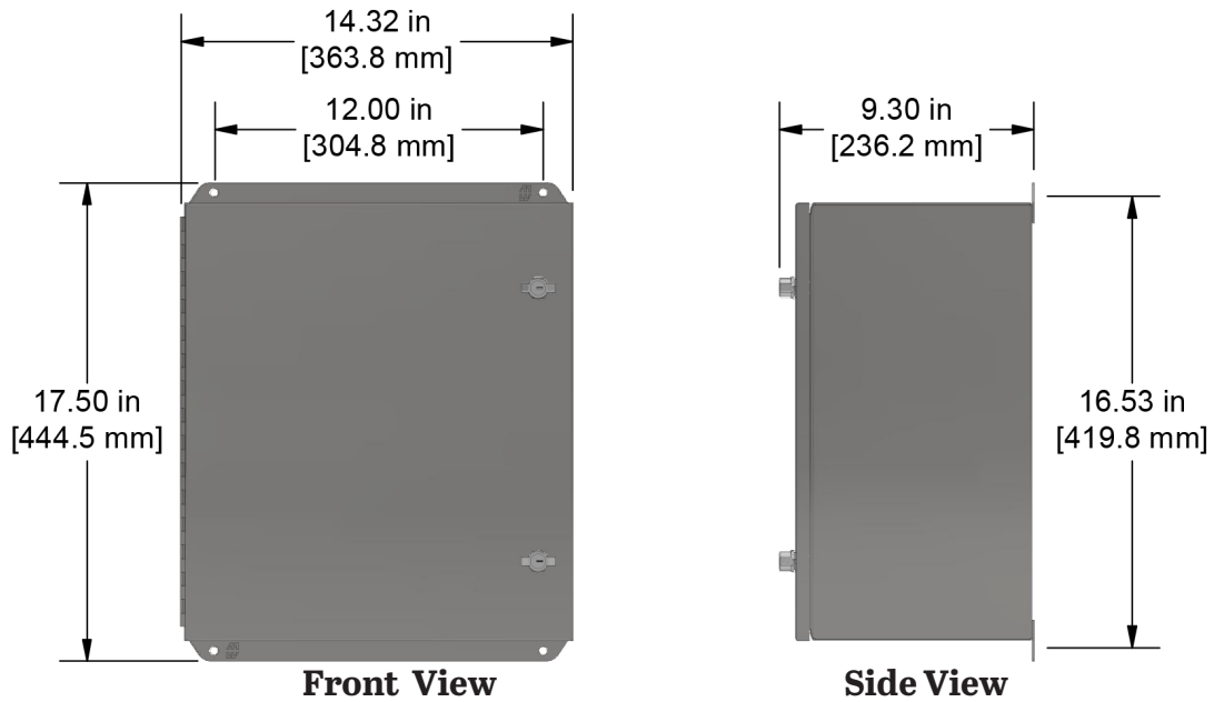
Figure 1. Dimensions
