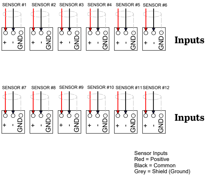
Figure 10. Field Wiring for Two-Conductor Sensor Inputs
