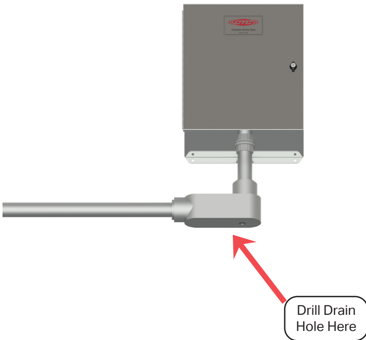
Figure 4. Conduit Entry for Switch Box
