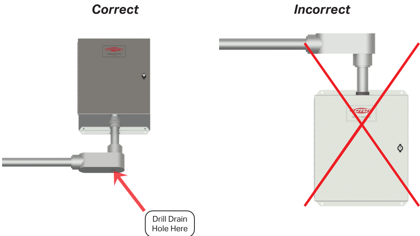
Figure 4. Conduit Entry for Switch Box
