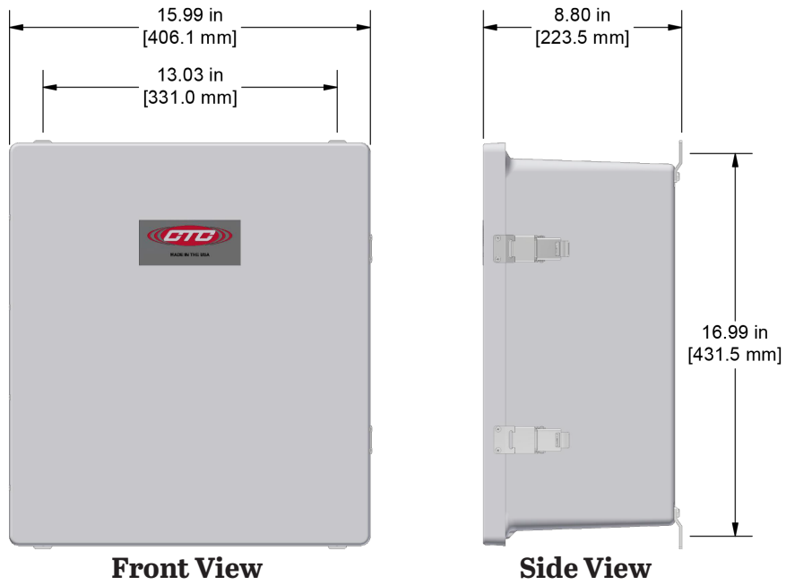
Figure 1. Dimensions
